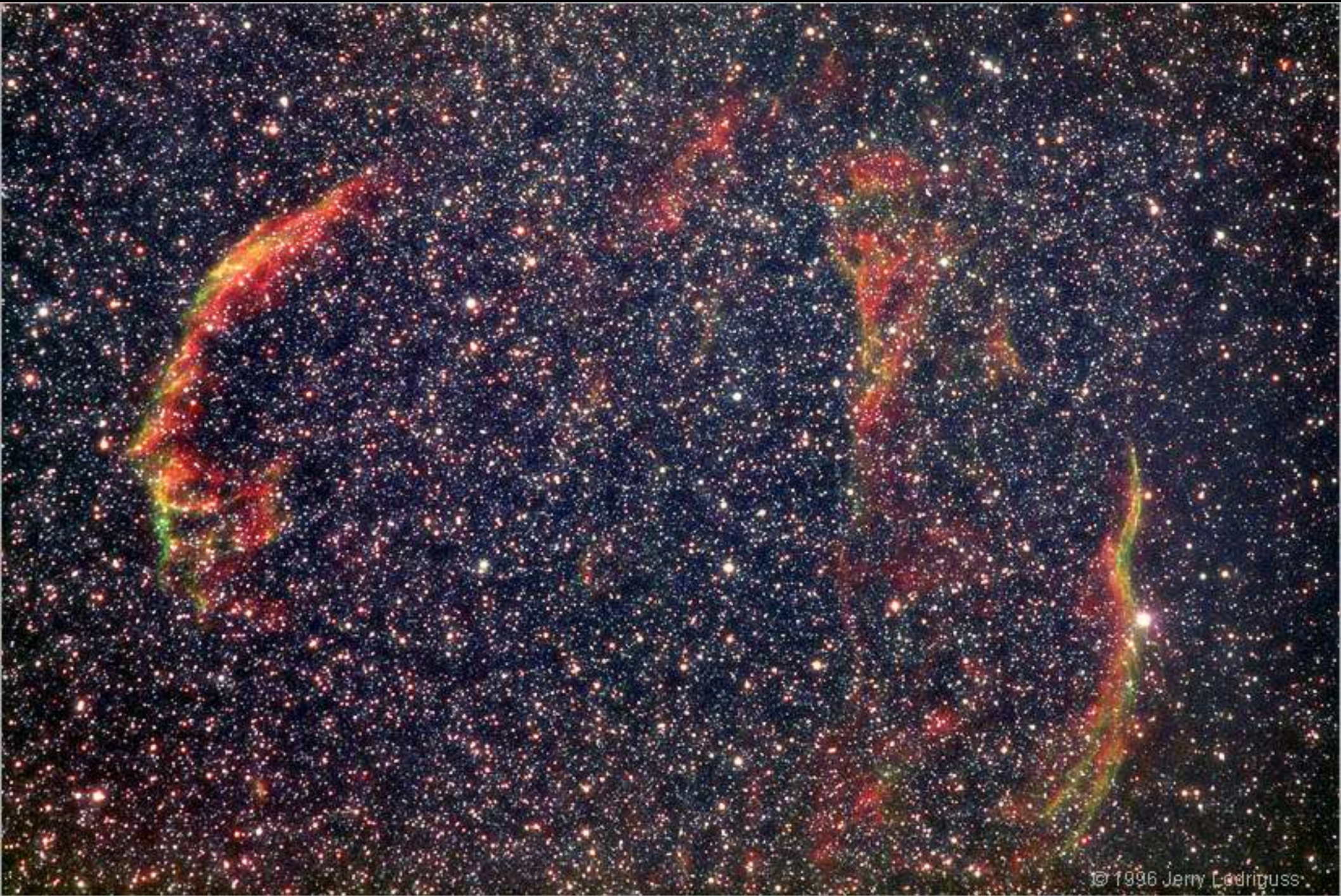
Veil nebula – 10,000 year old SNR, shock speed \sim 140 km/s
